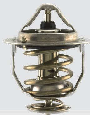
Bottom-By-Pass
