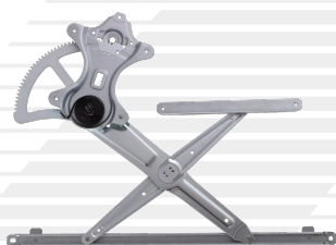
Regulator Only (Power) AISIN Prefix: RP-XXX
