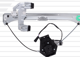
Power Regulator & Motor Assembly (Power) AISIN Prefix: RPA-XXX
